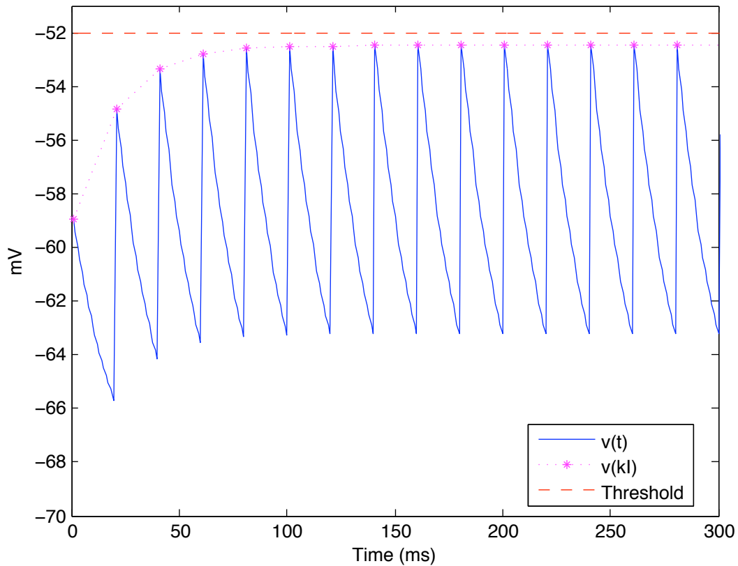
Voltage, ( I=20 ms, w_{inp}=11 mV)
